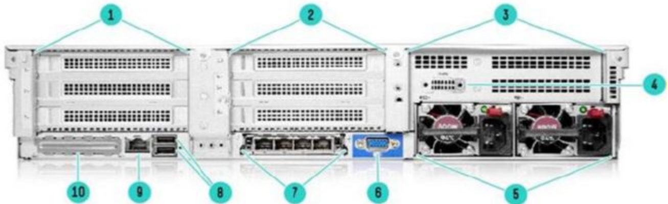
Rear View - Standard for all DL380 Gen10 Plus
