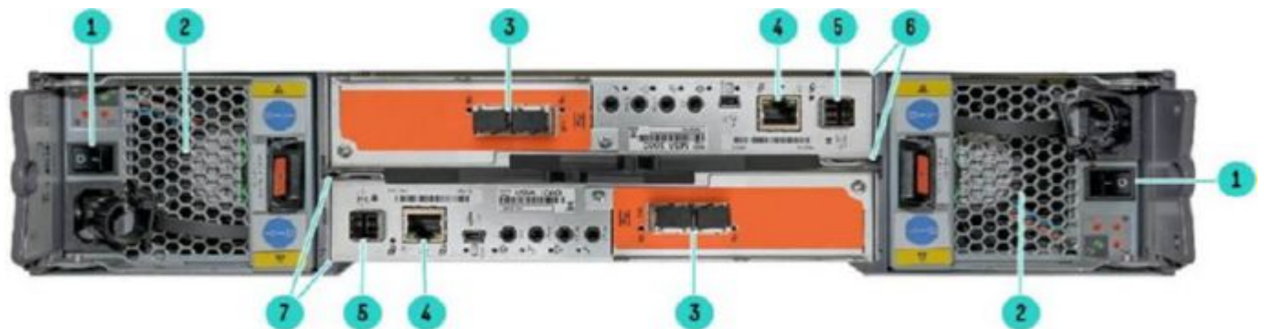
HPE MSA 1060 Storage-Rear View
