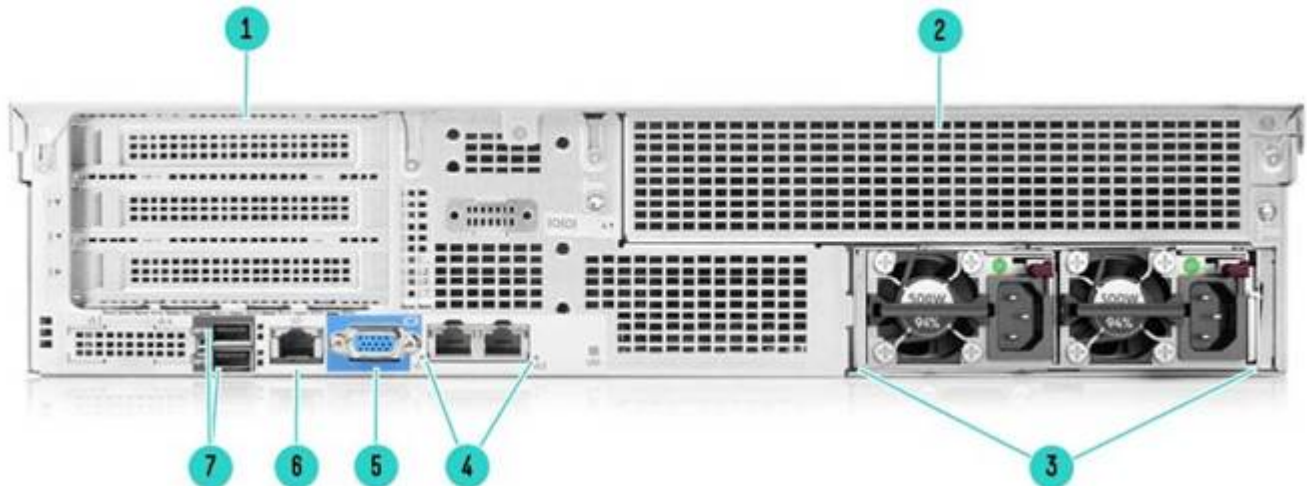
Rear View
